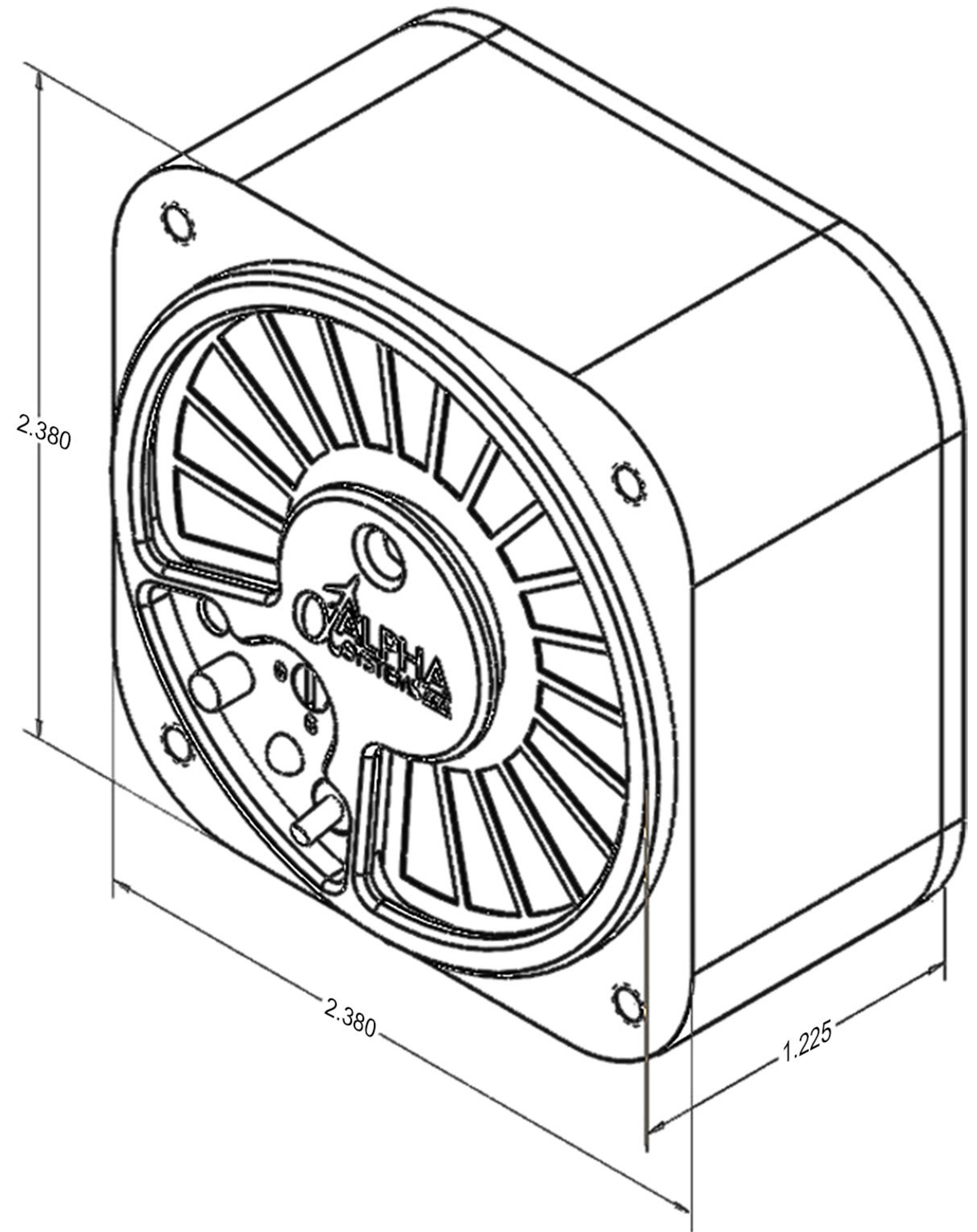
Condor Display Drawing with Measurements
