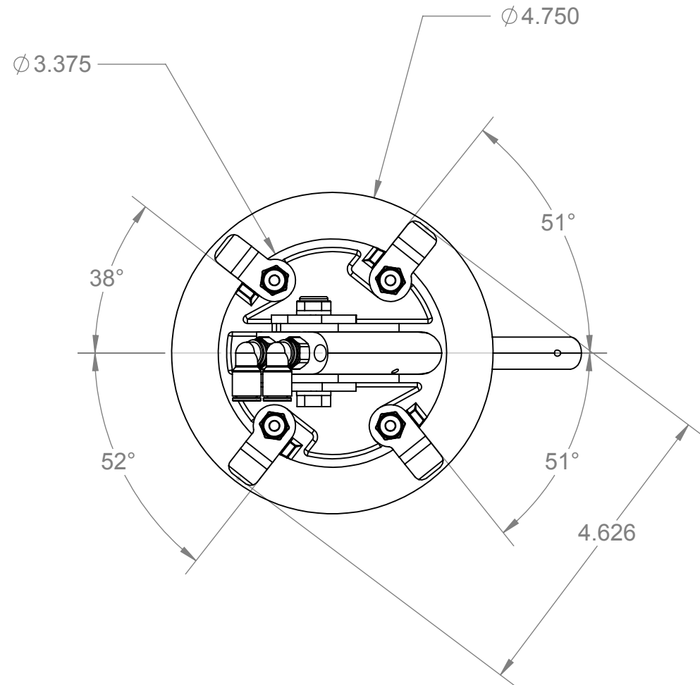
FRONT AND TOP VIEWS 1:2 SCALE
