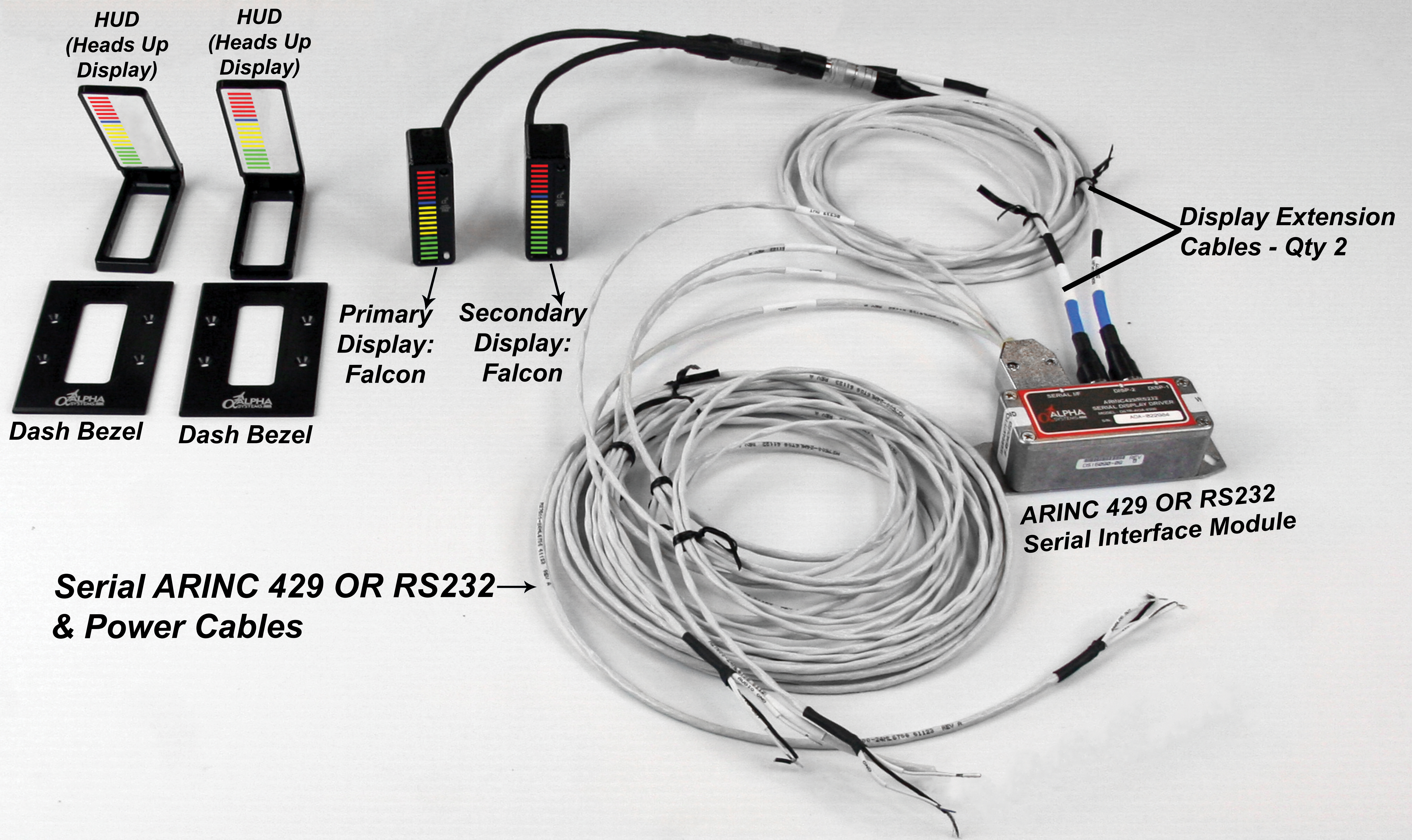
Alpha Systems AOA Raven Dual Falcon & HUD Connection Diagram
